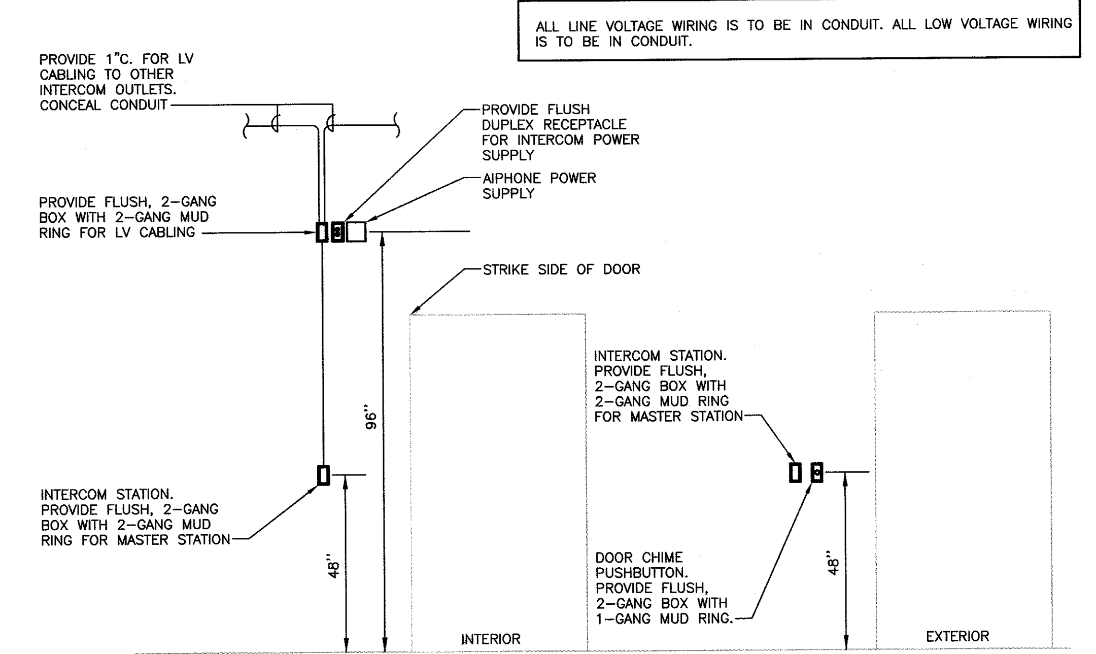
(2B) DEVICE ROUGH-IN PLAN
